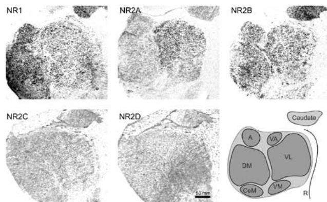
Figure 1 Transcript expression of NMDA receptor subunits NR1, NR2A-D in the human thalamus. NR1 transcripts were heavily expressed across the thalamus. There were also fairly high levels of NR2B transcripts, moderate levels of NR2A, and very low levels of NR2C and NR2D transcripts. In each section, the following nuclei were identified for each subject: anterior (A); central medial (CM); dorsomedial (DM); ventral anterior (VA); ventral lateral (VL); ventral medial (VM), and the reticular nucleus (R). The tail of the caudate nucleus is also readily apparent at this level.
